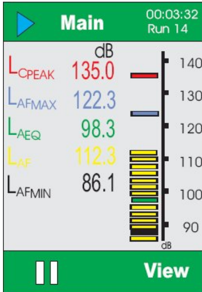
Example of main RUN screen for CEL-620.B Wide range integrating octave band analyzer
